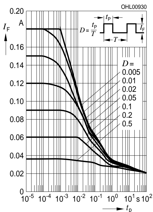
Zulässige Impulsbelastbarkeit I_F = f(t_p) Permissible Pulse Handling Capability Duty cycle D = parameter, T_A = 25\text{ °C} true green (3 Chips on)
